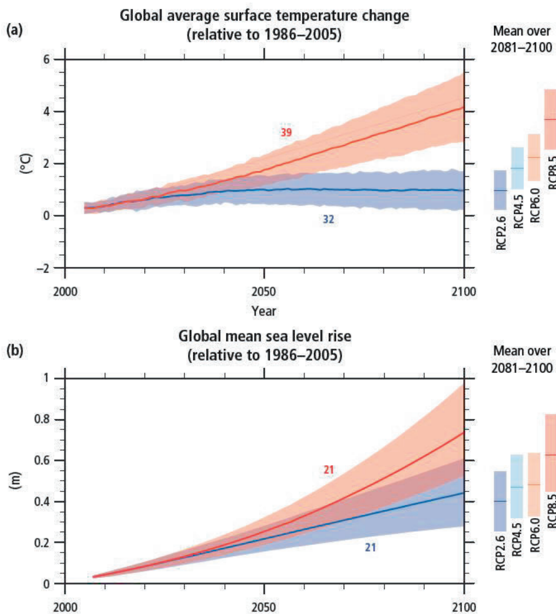
Figure 3. Increases in globally averaged (a) surface temperature and (b) sea level projected by the IPCC RCPs
