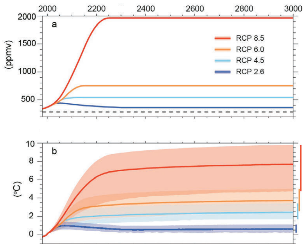
Figure 4. (a) Projected atmospheric CO 2 concentrations and (b) projected global mean surface temperature increase for the RCPs
