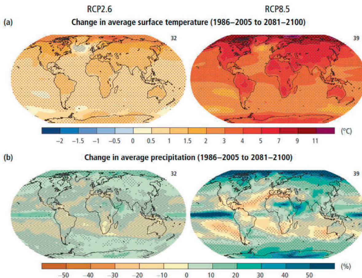
Figure 5. Change in average annual surface temperature (a) and change in average annual precipitation (b) based on multi-model mean projections for 2081–2100 relative to 1986–2005 under the RCP2.6 (left) and RCP8.5 (right) scenarios
